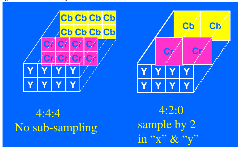
Figure 6 Color Subsampling
